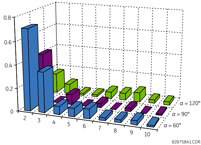
Figure 4: Harmonic content of the idealized inrush current for \alpha = 60^\circ, 90^\circ, and 120^\circ
